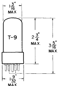
GLASS BULB
