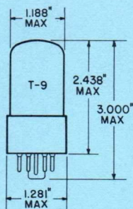
GLASS BULB INTERMEDIATE SHELL 8 PIN OCTAL B8-6 LOW LOSS PHENOLIC OUTLINE DRAWING JEDEC 9-5
