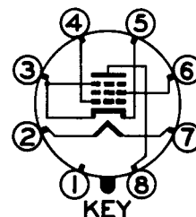
RMA 8BK BOTTOM VIEW
