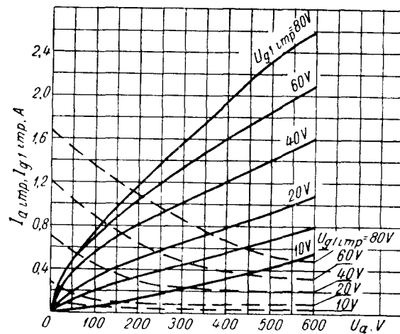
I_{a \text{ imp}}, I_{g1 \text{ imp}} = f(U_a) (триодное включение) (triode connection) — I_{a \text{ imp}} U_h = 6,3 \text{ V} - - - I_{g1 \text{ imp}} f_{\text{imp}} = 100 \text{ kHz} \tau = 2 \mu\text{s}
