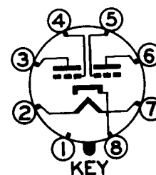
RMA 8B BOTTOM VIEW
