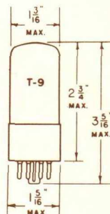
6N7GT/G
