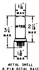
METAL SHELL 8 PIN OCTAL BASE
