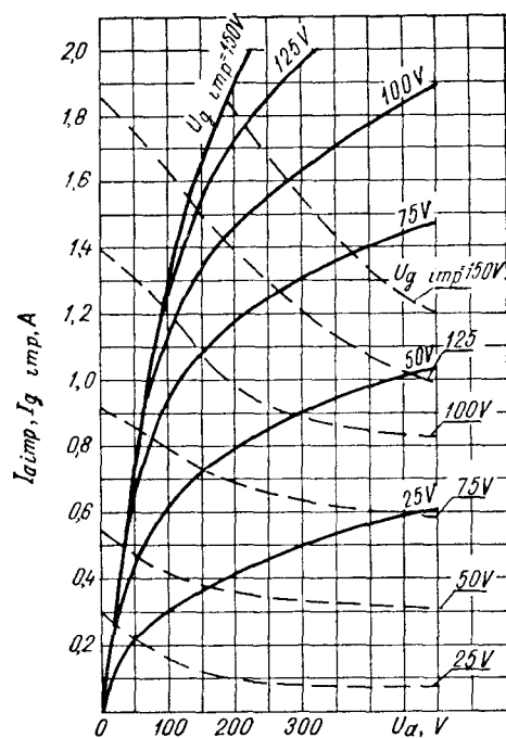
I_{a \text{ imp}}, I_{gT \text{ imp}} = f(U_a) (каждого триода) (for each triode) — I_{a \text{ imp}} U_h = 6,3 \text{ V} - - - I_{gT \text{ imp}} f_{\text{imp}} = 1 \text{ kHz} \tau = 2 \mu\text{s}
