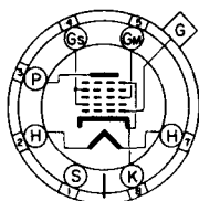
BOTTOM VIEW 6L7
