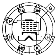
BOTTOM VIEW 6L7G
