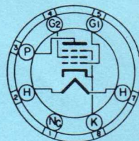
BOTTOM VIEW SHORT INTERMEDIATE SHELL 7 PIN LOW LOSS PHENOLIC
