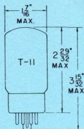
GLASS BULB
