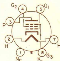
BOTTOM VIEW BASING DIAGRAM JEDEC 75
