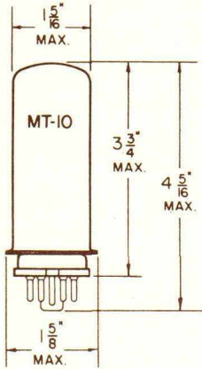
METAL SHELL
