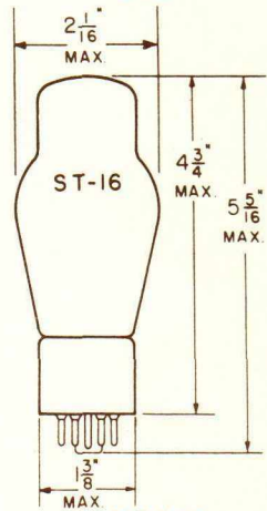
GLASS BULB
