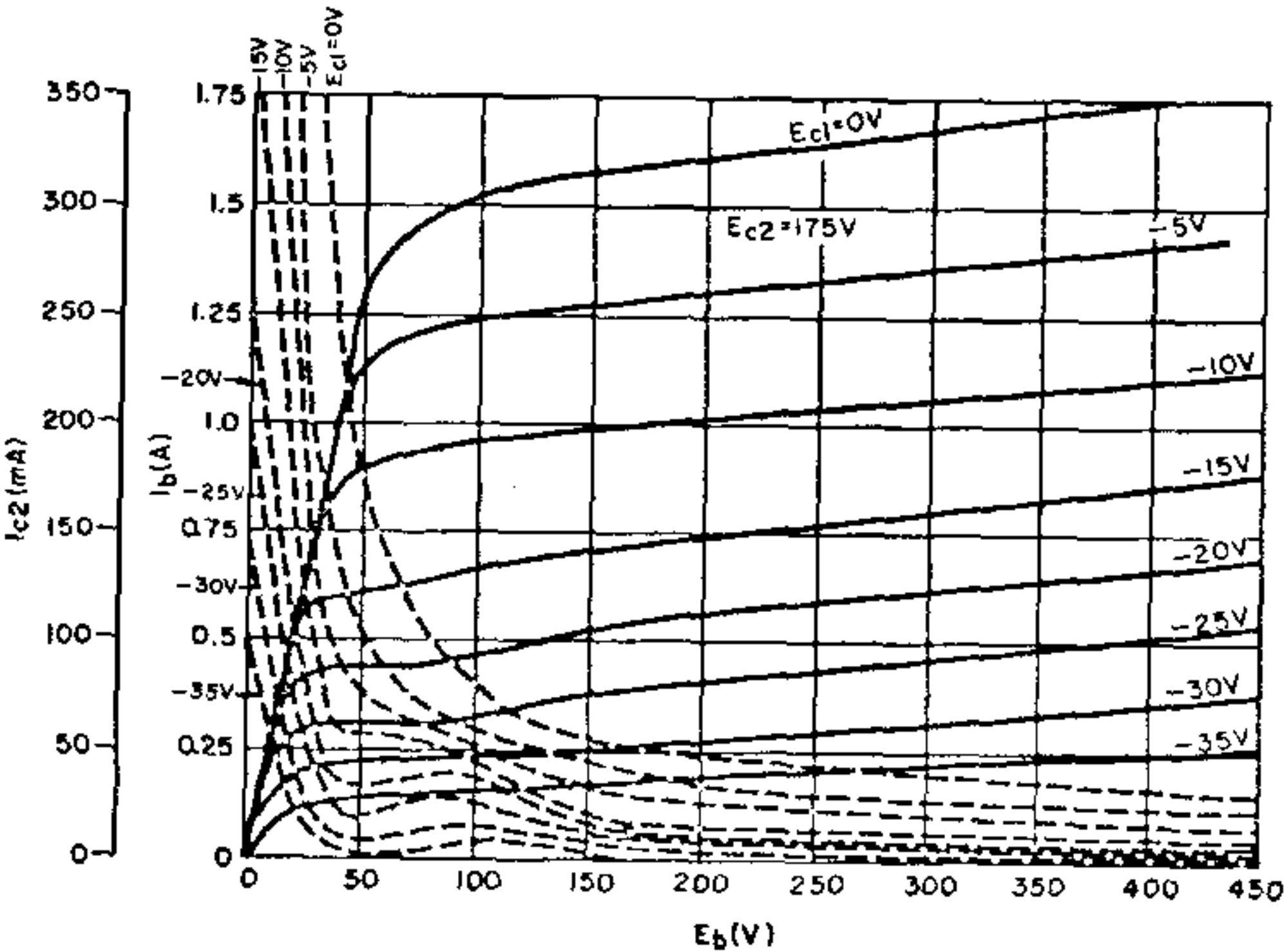
Plate Characteristics
