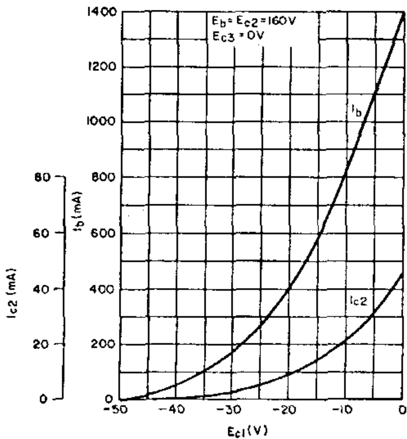
Transfer Characteristics
