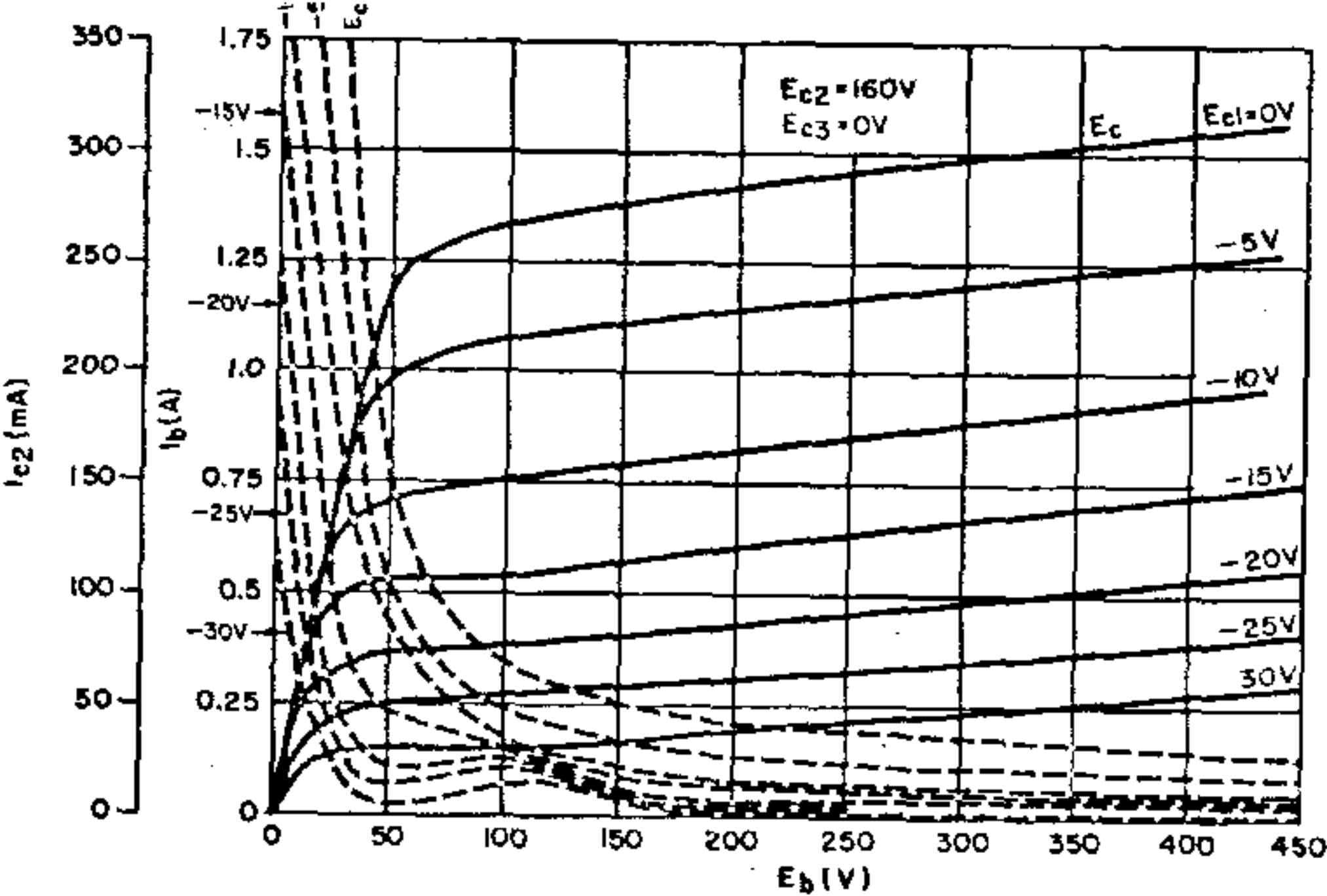
Plate Characteristics
