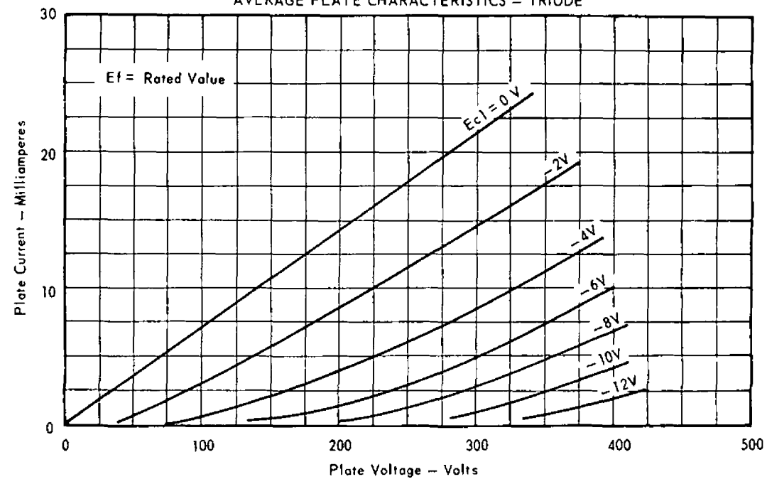
AVERAGE PLATE CHARACTERISTICS - TRIODE
