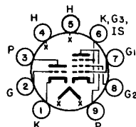
BOTTOM VIEW BASING DIAGRAM JEDEC 9DX
