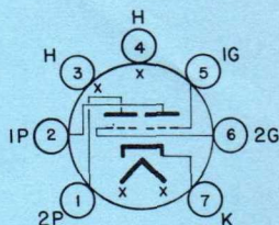
BOTTOM VIEW BASING DIAGRAM JEDEC 7BF
