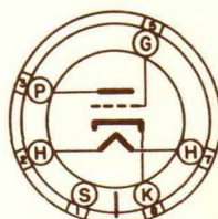
BOTTOM VIEW SMALL WAFER 6 PIN OCTAL METAL SLEEVE
