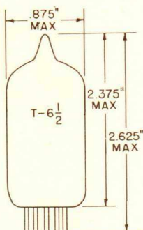
GLASS BULB SMALL BUTTON 9 PIN BASE E9-1 OUTLINE DRAWING JEDEC 6-3
