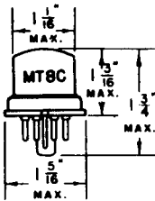
METAL SHELL 7 PIN OCTAL BASE 6H6
