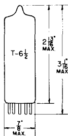
GLASS BULB
