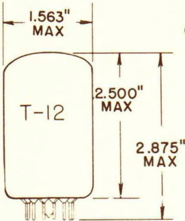
GLASS BULB
