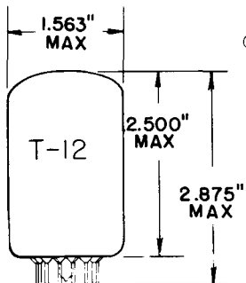
GLASS BULB BUTTON 12 PIN BASE E12-74 OUTLINE DRAWING JEDEC 12-56
