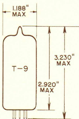
GLASS BULB
