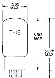
GLASS BULB SHORT MEDIUM SHELL 6 PIN OCTAL 86-112
