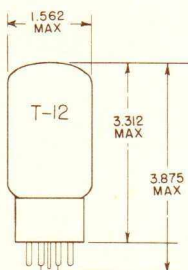
GLASS BULB SHORT MEDIUM SHELL 6 PIN OCTAL B6-112
