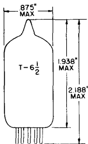
GLASS RULER SMALL BUTTON 9 PIN BASE EQ-1 OUTLINE DRAWING JEDEC A-2
