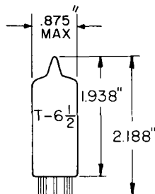
GLASS BULB 9 PIN BASE E9-2 OUTLINE DRAWING JEDEC 6-2
