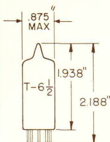
GLASS BULB 9 PIN BASE E9-1 OUTLINE DRAWING JEDEC 6-2
