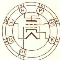
BOTTOM VIEW SMALL-BUTTON MINIATURE 7 PIN BASE 7FQ
