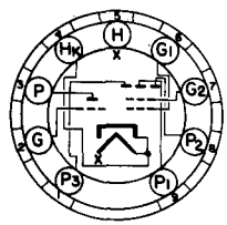
BOTTOM VIEW SMALL-BUTTON 9 PIN NOVAL 9KP
