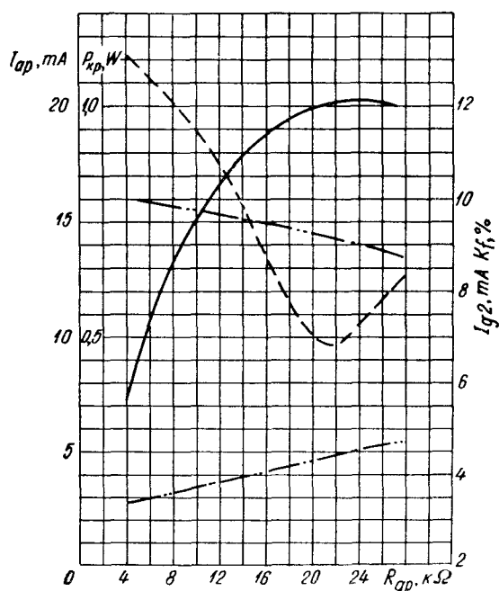
I_{ap}, I_{g2}, P_{kp}, k_{ip} = f(R_{ap}) \text{---} I_{ap} U_h = 6,3 \text{ V} \text{---} I_{g2} U_{ap} = 250 \text{ V} \text{---} P_{kp} U_{g2} = 200 \text{ V} \text{---} k_{ip} U_{g1} = -3 \text{ V} U_{g1 \sim (eff)} = 0,9 \text{ V}
