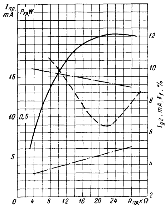
I_{ap}, I_{g2}, P_{kp}, k_{ip} = f(R_{ap}) \text{---} I_{ap} U_h = 6,3 \text{ V} \text{---} I_{g2} U_{ap} = 250 \text{ V} \text{---} P_{kp} U_{g2} = 240 \text{ V} \text{---} k_{ip} U_{g1} = -4,2 \text{ V} U_{g1 \sim (eff)} = 1 \text{ V}
