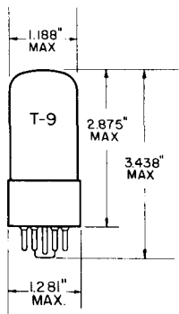
GLASS BULB INTERMEDIATE - SHELL 6 PIN OCTAL B6-81 OUTLINE DRAWING JEDEC 9-15
