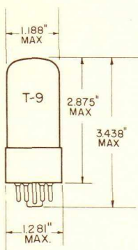
GLASS BULB INTERMEDIATE - SHELL 6 PIN OCTAL B6-81 OUTLINE DRAWING JEDEC 9-15
