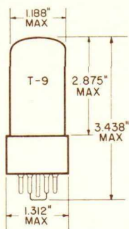
GLASS BULB INTERMEDIATE-SHELL 6 PIN OCTAL B6-81 AND B6-84 OUTLINE DRAWING JEDEC 9-15
