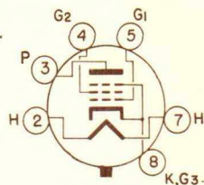
BOTTOM VIEW BASING DIAGRAM JEDEC 7AC
