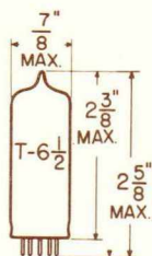
GLASS BULB
