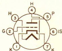
BOTTOM VIEW BASING DIAGRAM
