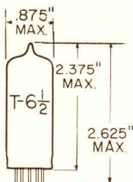
GLASS BULB SMALL BUTTON 9 PIN NOVAL E9-1
