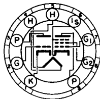
BOTTOM VIEW MINIATURE BUTTON 9 PIN BASE 90X
