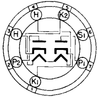
BOTTOM VIEW SMALL BUTTON MINIATURE 7 PIN BASE
