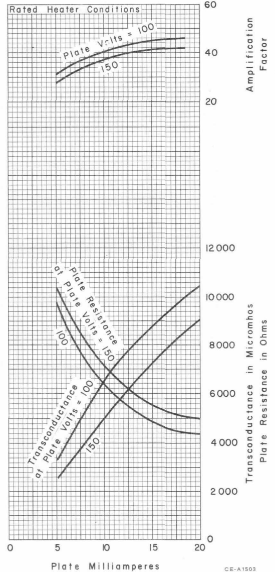
AVERAGE CHARACTERISTICS Triode Unit
