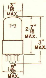
GLASS BULB INTERMEDIATE SHELL 8 PIN OCTAL BB-6 OUTLINE DRAWING JEDEC 9-5
