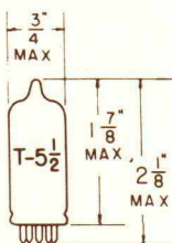
GLASS BULB
