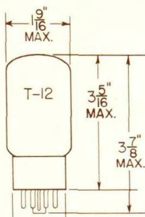
GLASS BULB
