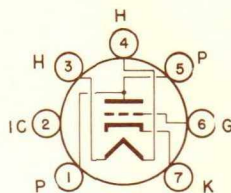
BOTTOM VIEW BASING DIAGRAM JEDEC 6BG
