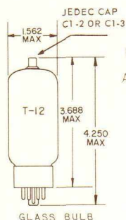
SKIRTED MINIATURE SHORT MEDIUM-SHELL 6 PIN OCTAL B6-122, B6-148 OR 7 PIN OCTAL B7-111, B7-119 OR B5-190 ← OUTLINE DRAWING JEDEC 17-51
