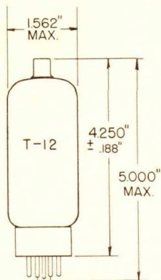
GLASS BULB SMALL CAP SMALL MEDIUM-SHELL 8 PIN OCTAL B8-118 WITH EXTERNAL BARRIERS STYLE B OUTLINE DRAWING JEDEC 12-22
