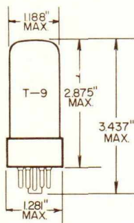
GLASS BULB SHORT INTERMEDIATE SHELL 5 PIN OCTAL B5-B5 OUTLINE DRAWING JEDEC 9-43
