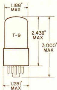
GLASS BULB INTERMEDIATE-SHELL 8 PIN OCTAL 88-142 OUTLINE DRAWING JEDEC 9-5
