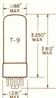
GLASS BULB
