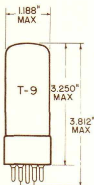
GLASS BULB JEDEC GROUP 1 B5-B5 SHORT INTERMEDIATE-SHELL 5 PIN OCTAL WITH EXTERNAL BARRIERS
